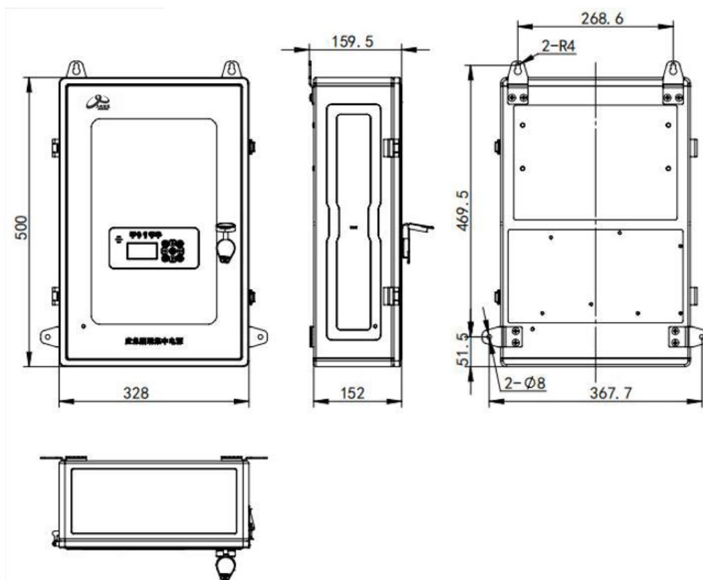
JF-D-AC(DC36V/0.25kVA)-DA105(65)外形尺寸示意图
