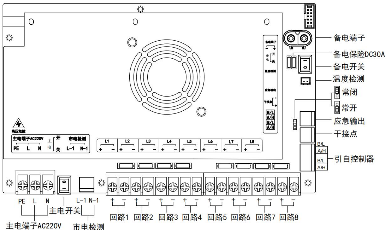
JF-D-AC(DC36V/0.25kVA)-DA105(65)接线端子示意图
